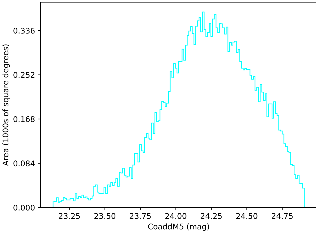
too_5_4v3.4_10yrs Yr 1 u band: CoaddM5
