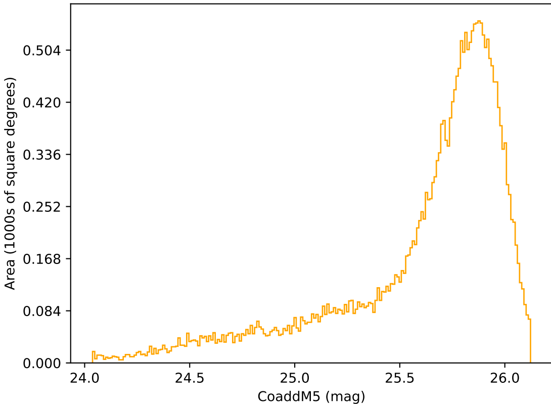
too_5_4v3.4_10yrs Yr 1 r band: CoaddM5
