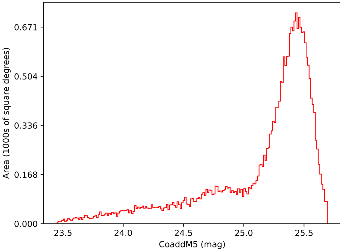
too_5_4v3.4_10yrs Yr 1 i band: CoaddM5
