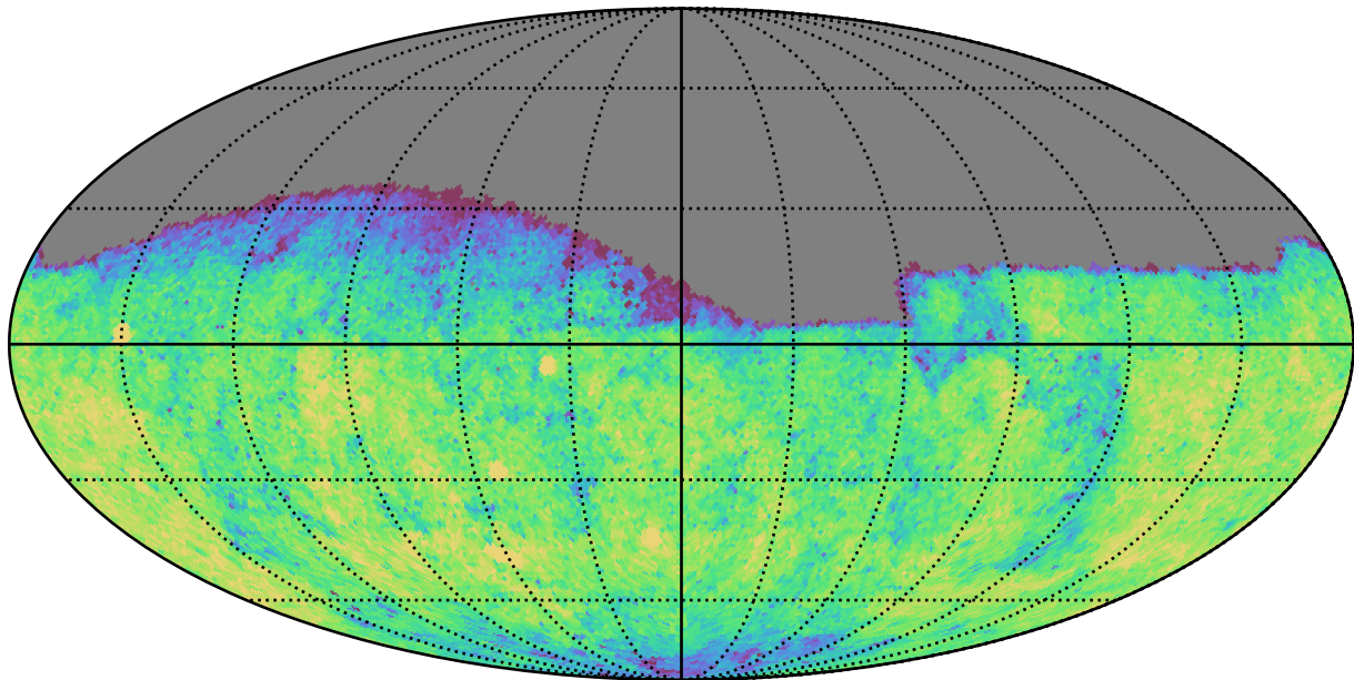
too_5_4v3.4_10yrs Yr 1 g band: CoaddM5
