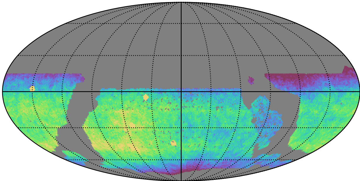
too_5_4v3.4_10yrs WFD z band: CoaddM5
