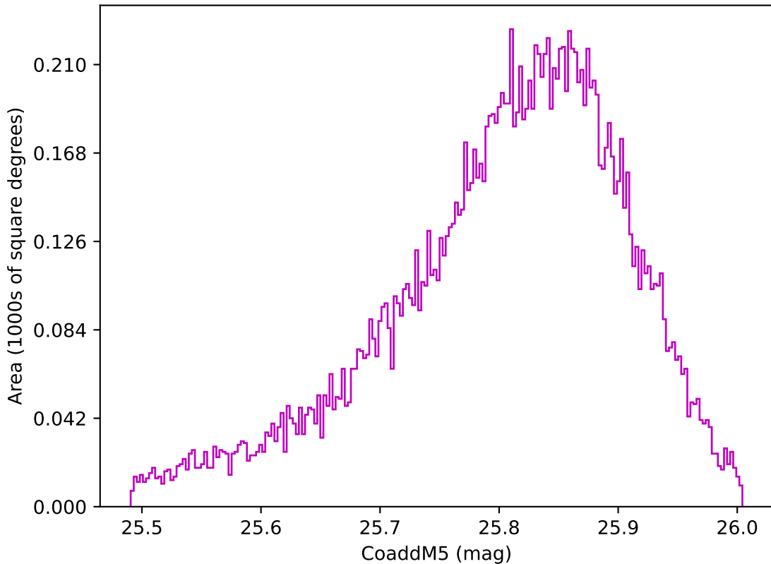
too_5_4v3.4_10yrs WFD z band: CoaddM5
