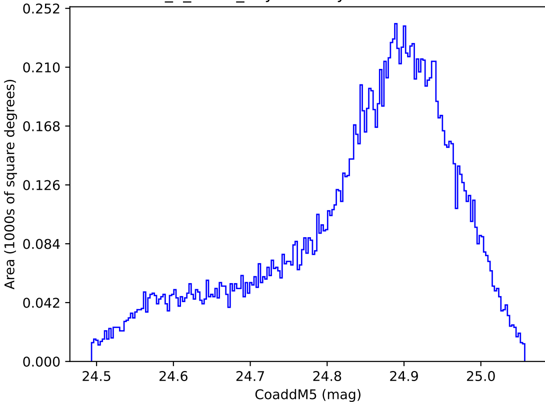
too_5_4v3.4_10yrs WFD y band: CoaddM5
