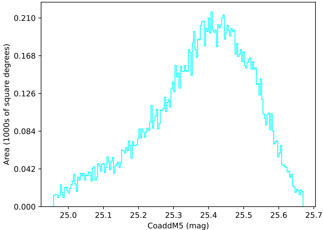
too_5_4v3.4_10yrs WFD u band: CoaddM5
