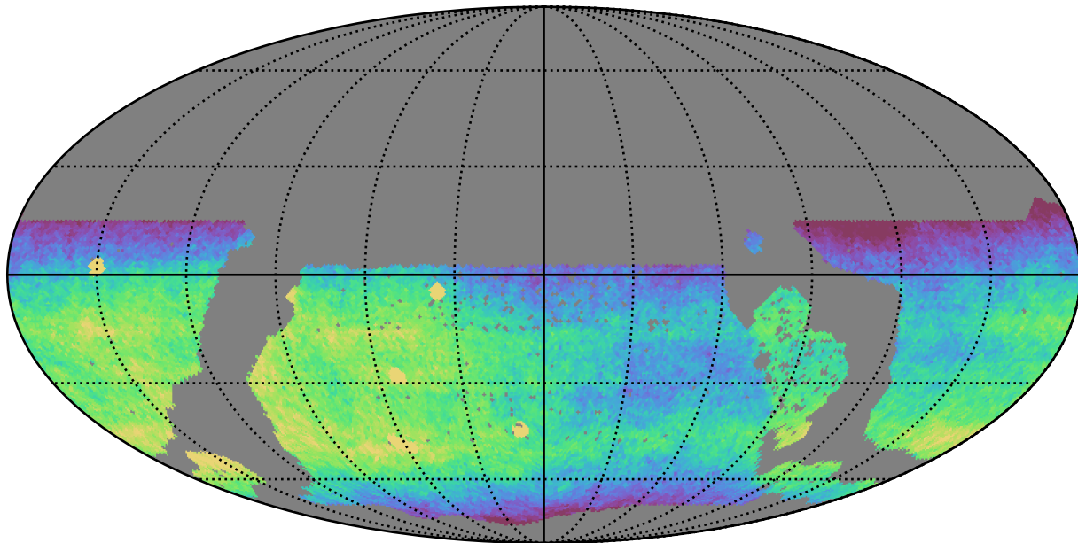
too_5_4v3.4_10yrs WFD r band: CoaddM5
