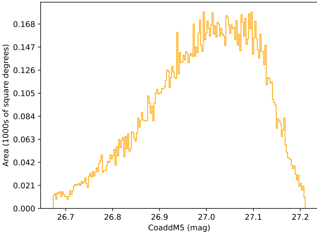
too_5_4v3.4_10yrs WFD r band: CoaddM5
