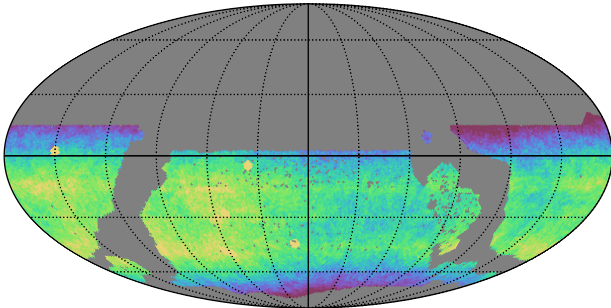
too_5_4v3.4_10yrs WFD i band: CoaddM5
