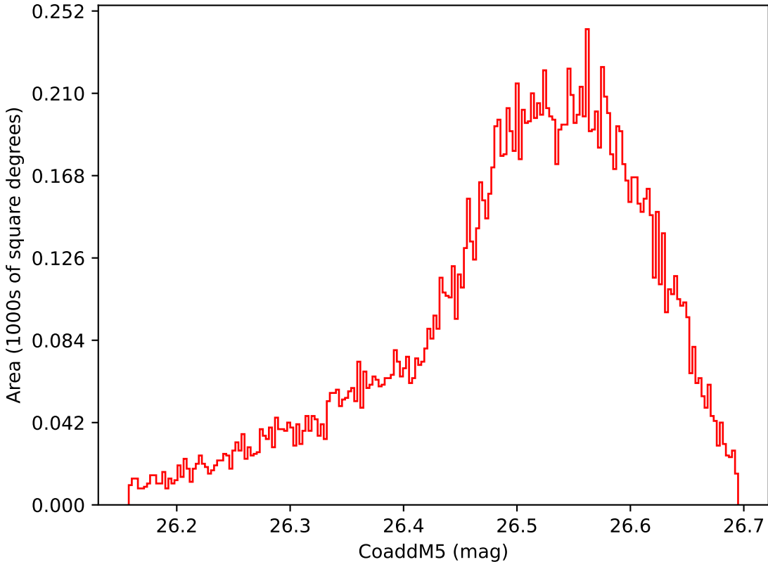
too_5_4v3.4_10yrs WFD i band: CoaddM5
