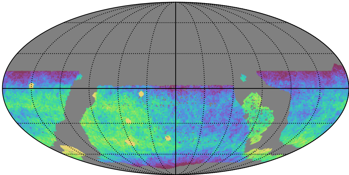
too_5_4v3.4_10yrs WFD g band: CoaddM5
