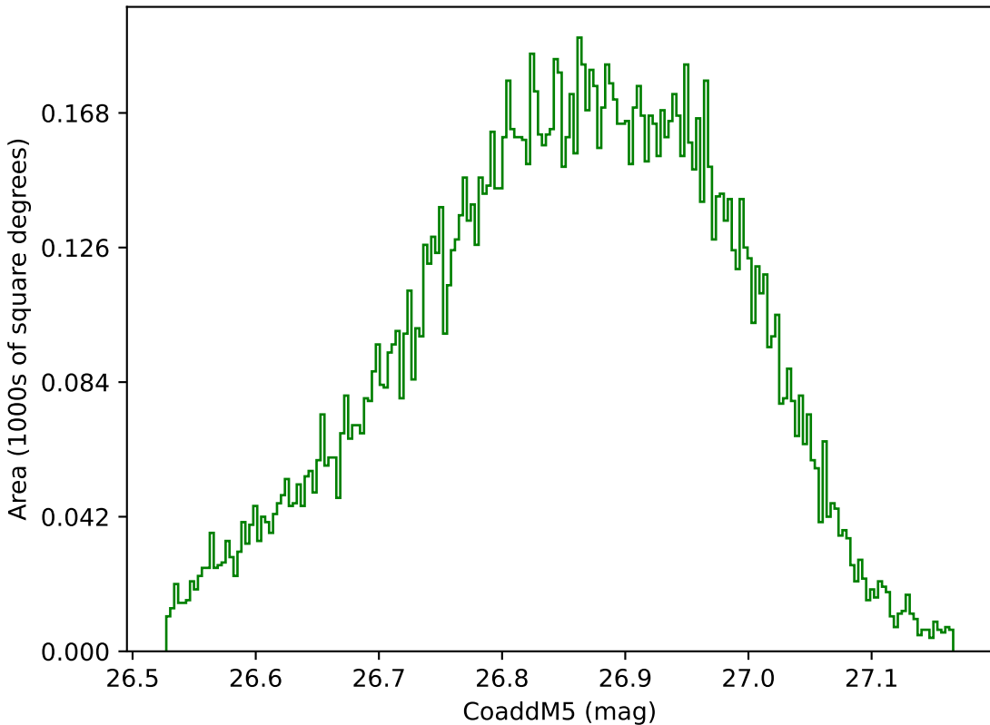
too_5_4v3.4_10yrs WFD g band: CoaddM5
