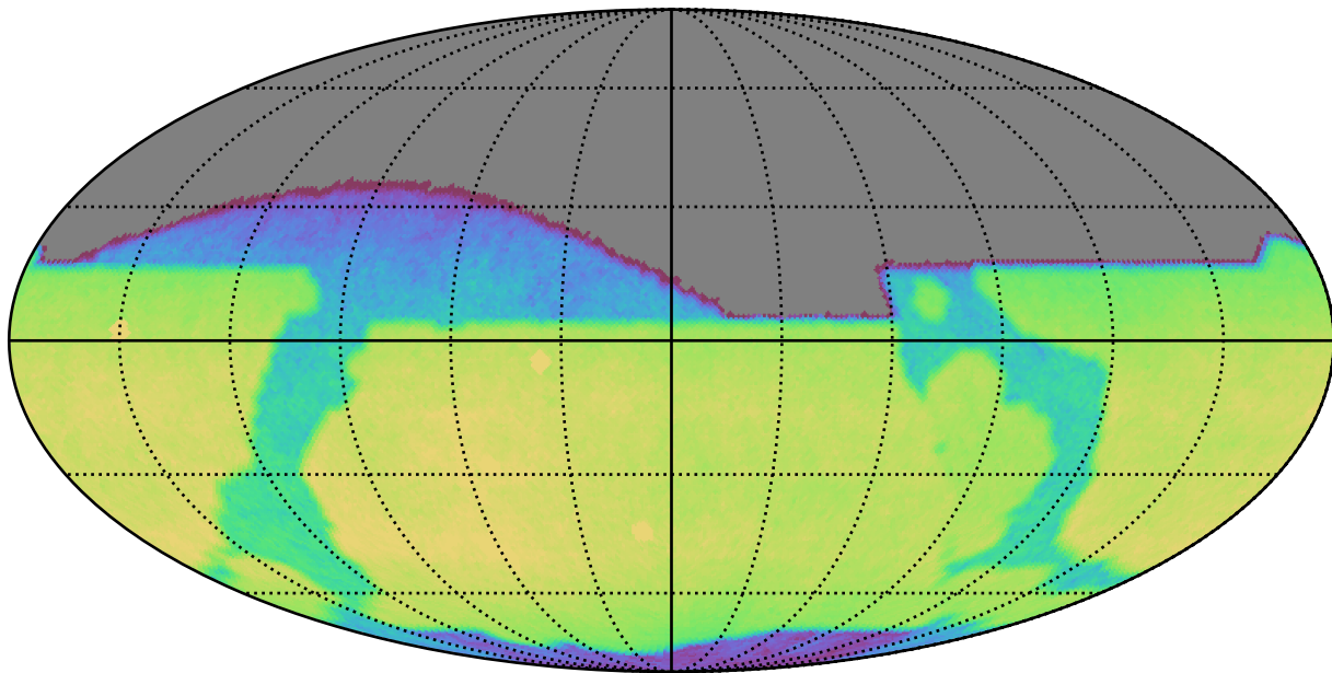
too_5_4v3.4_10yrs All sky z band: CoaddM5
