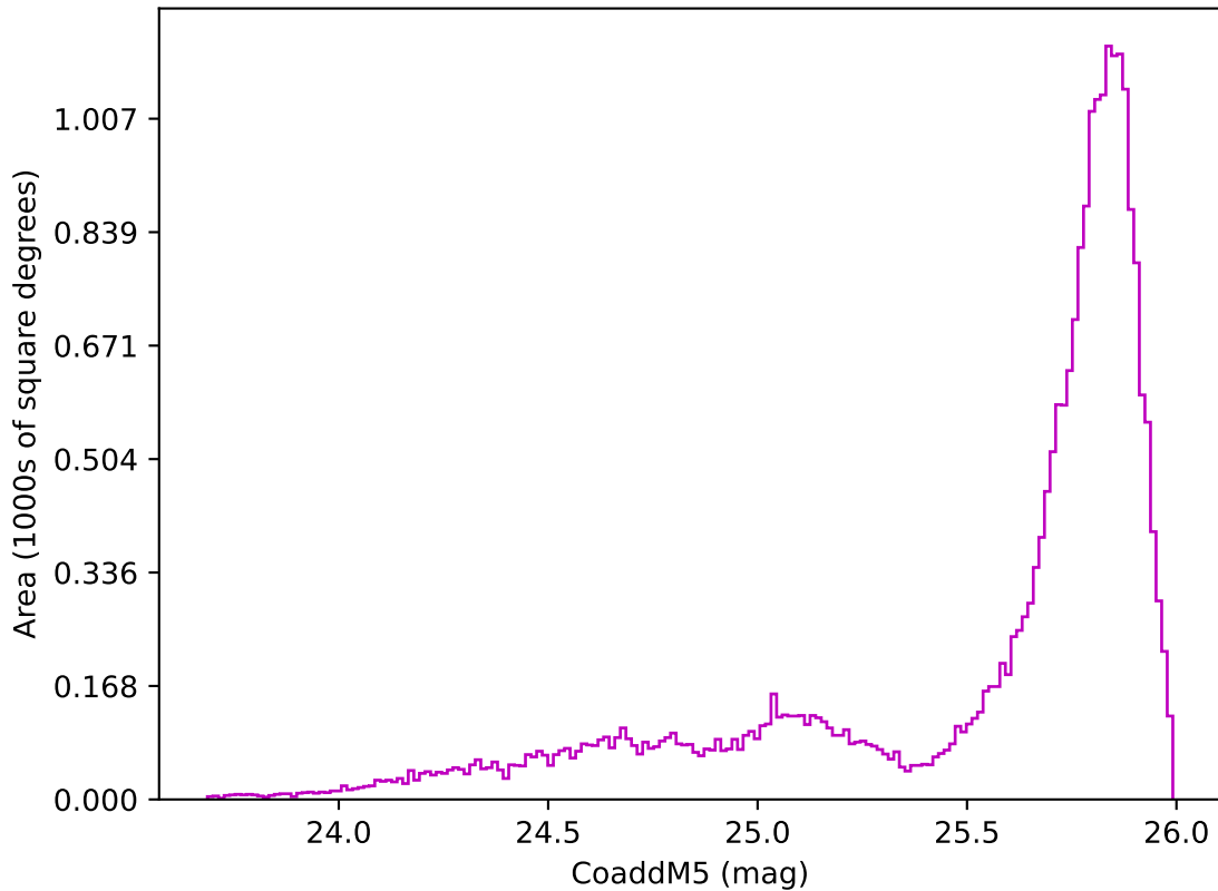
too_5_4v3.4_10yrs All sky z band: CoaddM5
