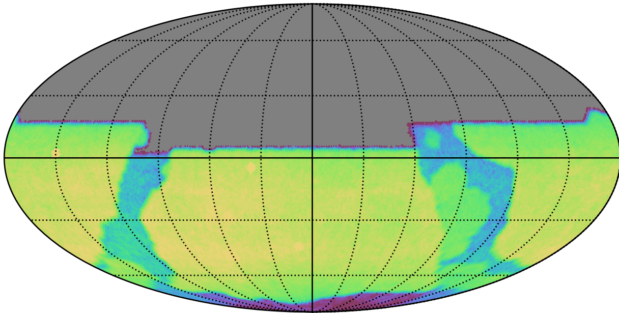
too_5_4v3.4_10yrs All sky y band: CoaddM5
