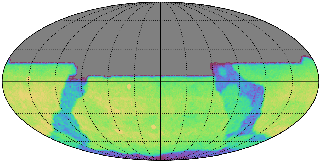
too_5_4v3.4_10yrs All sky u band: CoaddM5
