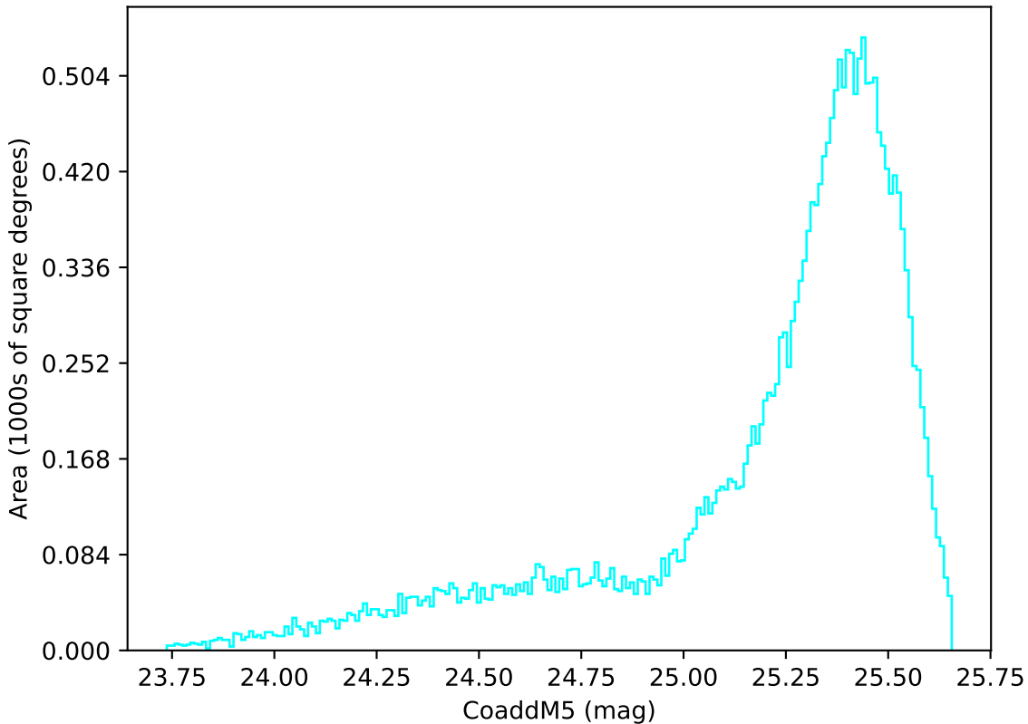
too_5_4v3.4_10yrs All sky u band: CoaddM5
