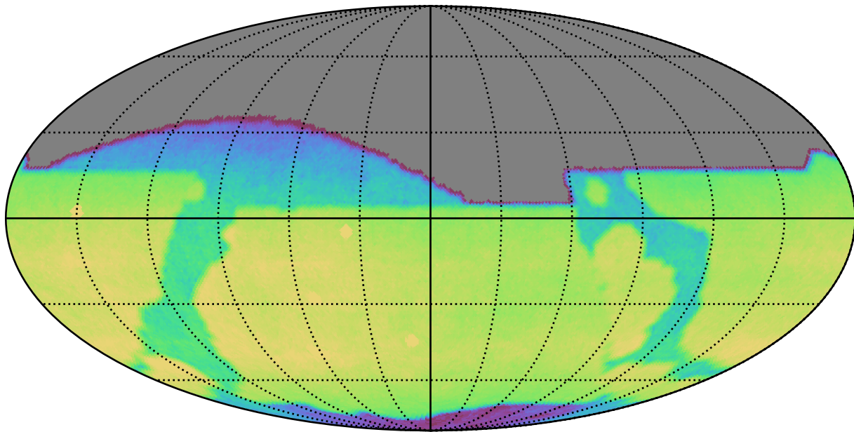
too_5_4v3.4_10yrs All sky r band: CoaddM5
