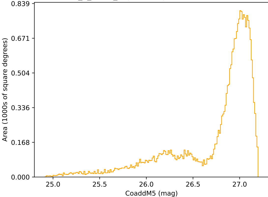
too_5_4v3.4_10yrs All sky r band: CoaddM5
