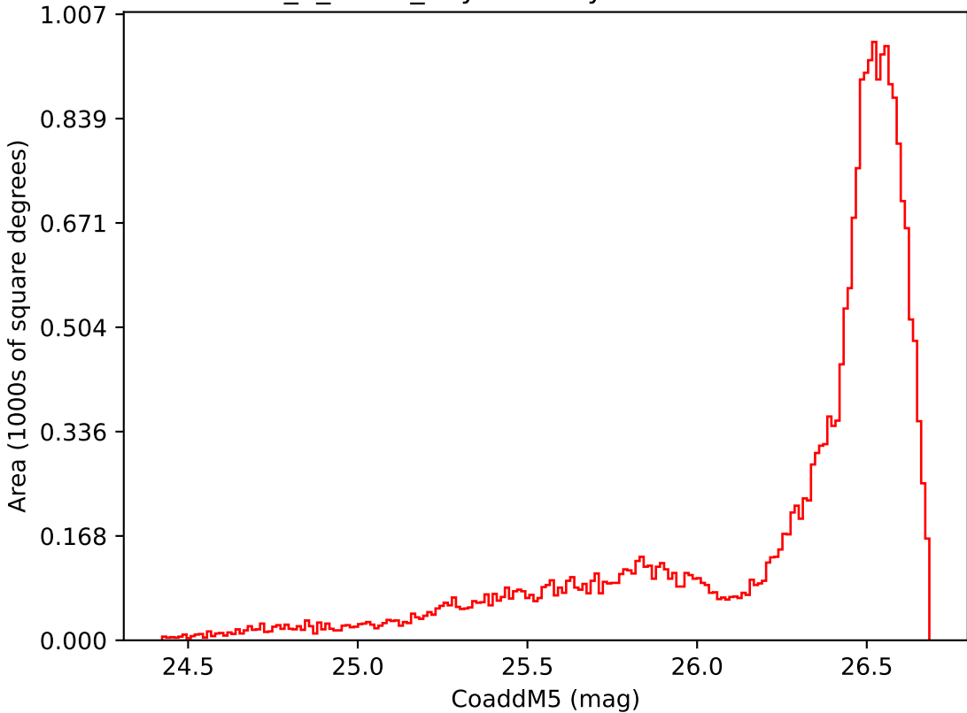
too_5_4v3.4_10yrs All sky i band: CoaddM5
