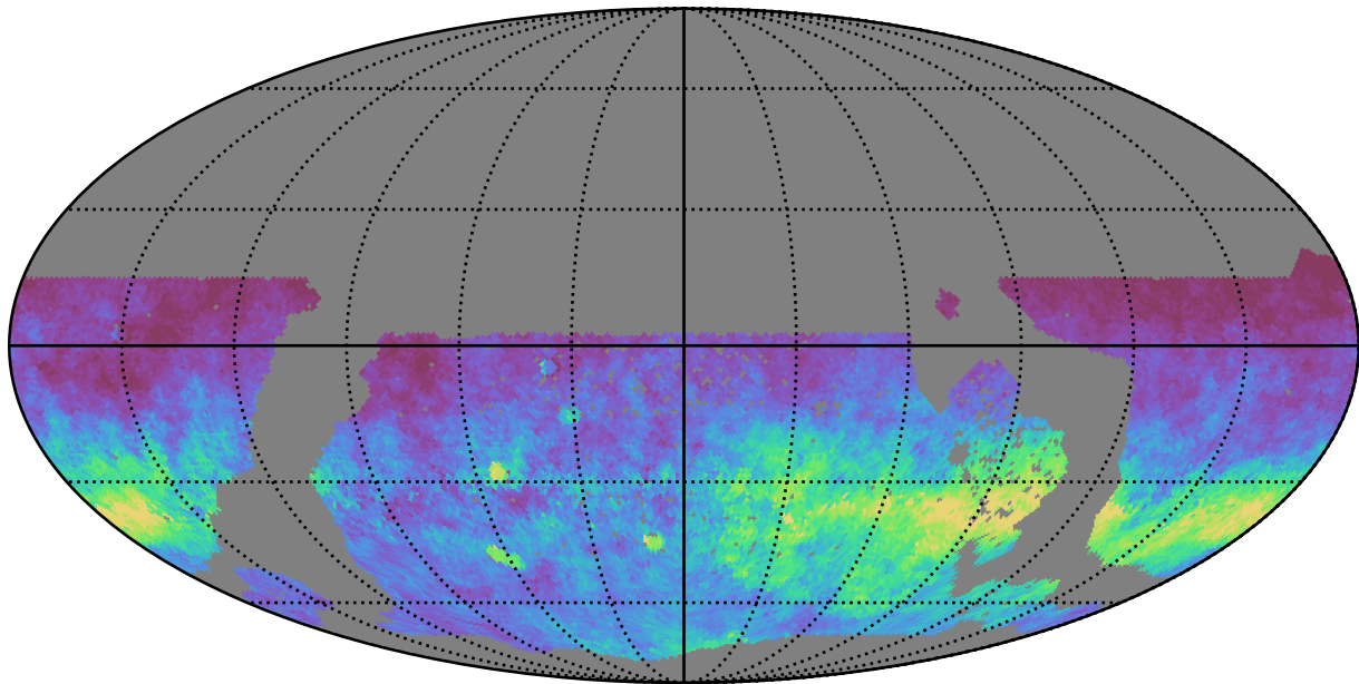
too_5_4v3.4_10yrs WFD z band: AngleRms rotSkyPos
