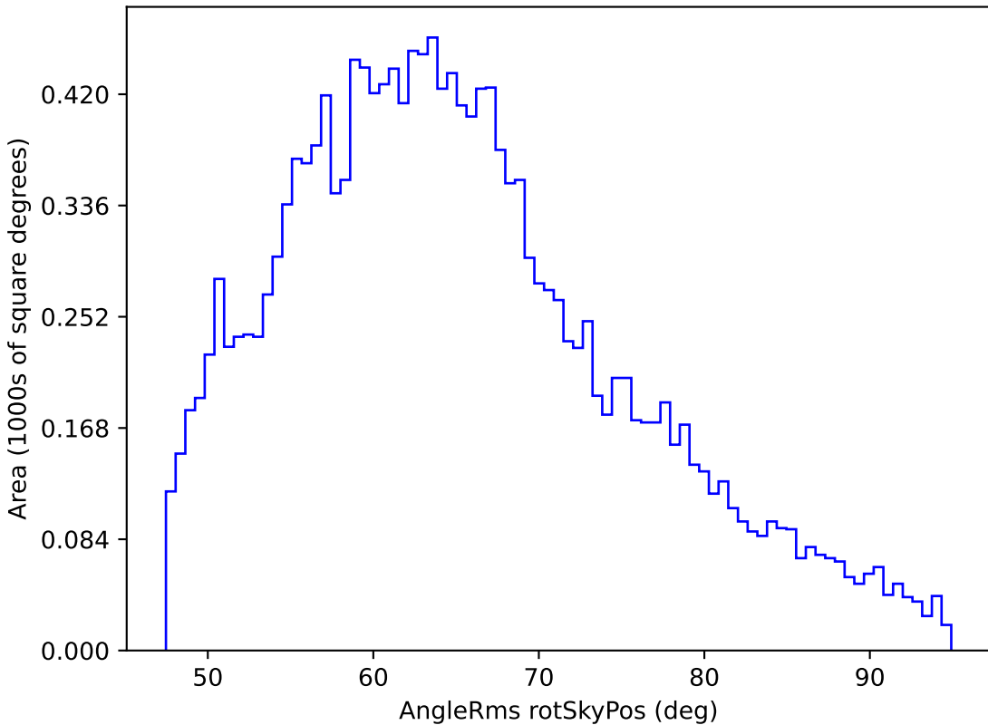
too_5_4v3.4_10yrs WFD z band: AngleRms rotSkyPos
