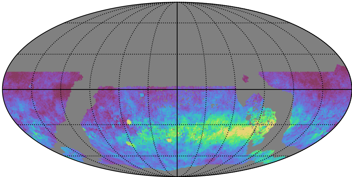
too_5_4v3.4_10yrs WFD y band: AngleRms rotSkyPos
