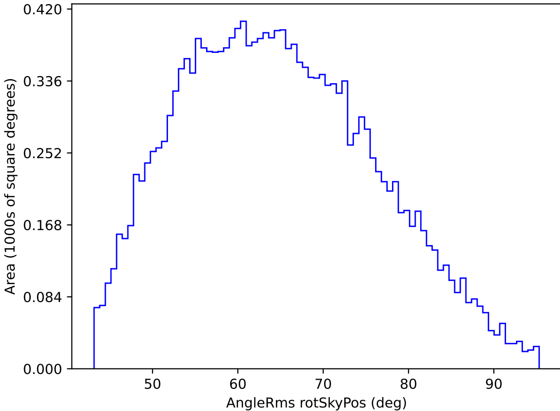
too_5_4v3.4_10yrs WFD u band: AngleRms rotSkyPos
