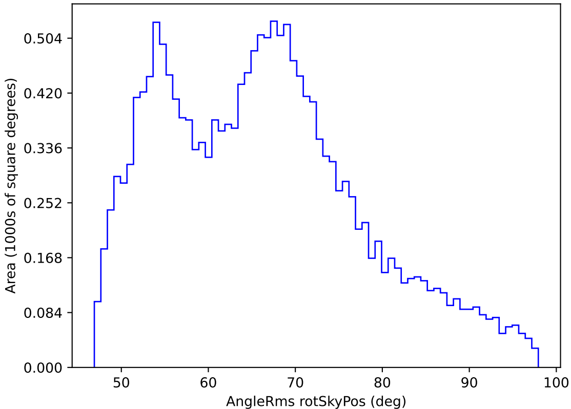
too_5_4v3.4_10yrs WFD r band: AngleRms rotSkyPos
