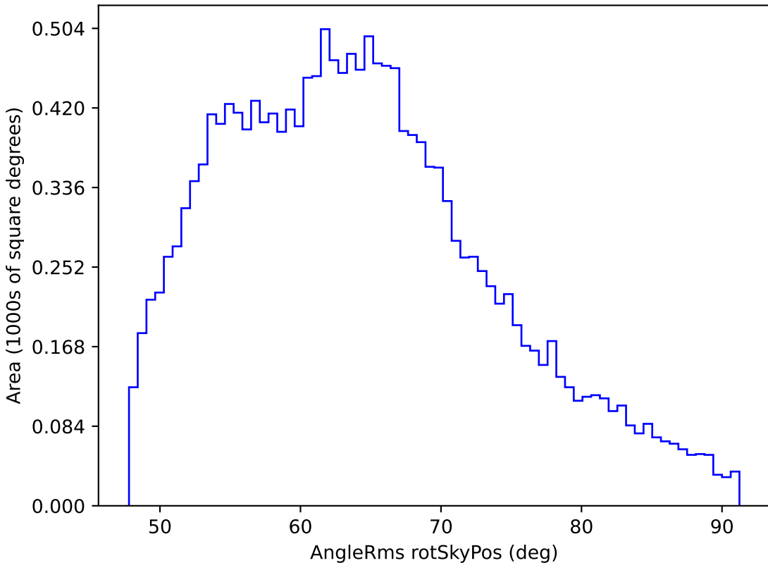
too_5_4v3.4_10yrs WFD i band: AngleRms rotSkyPos
