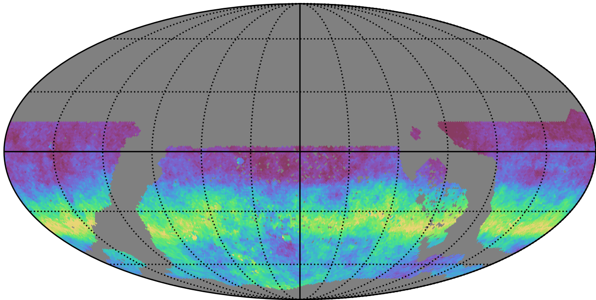
too_5_4v3.4_10yrs WFD g band: AngleRms rotSkyPos
