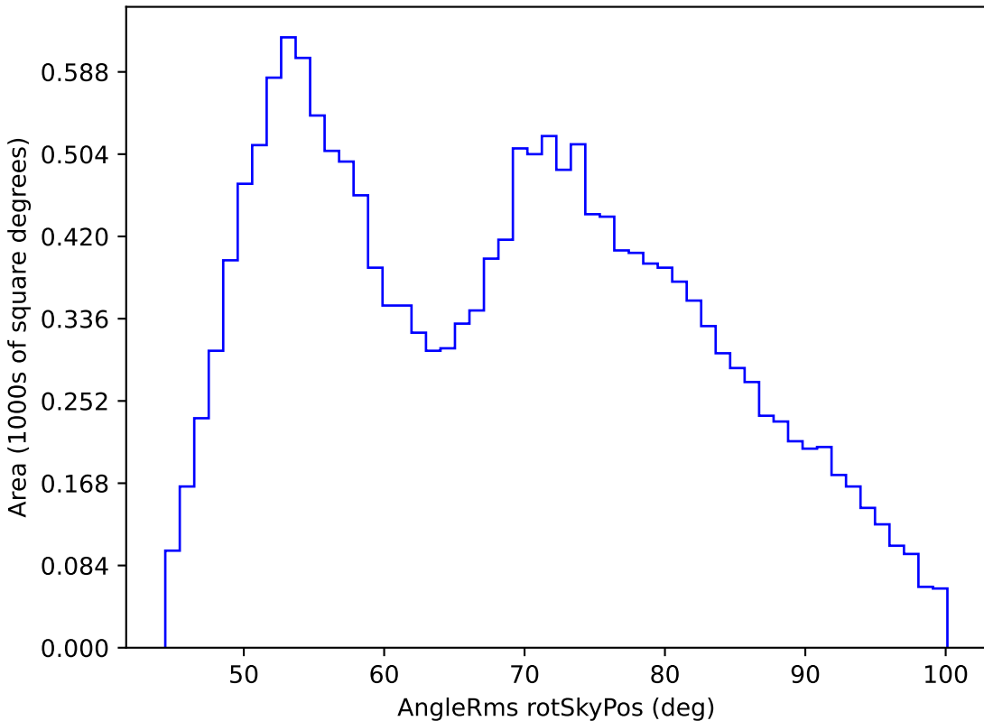
too_5_4v3.4_10yrs WFD g band: AngleRms rotSkyPos
