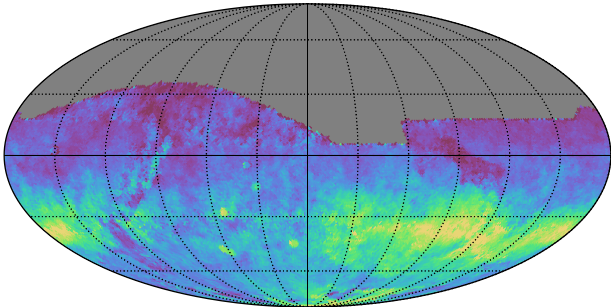
too_5_4v3.4_10yrs All sky z band: AngleRms rotSkyPos
