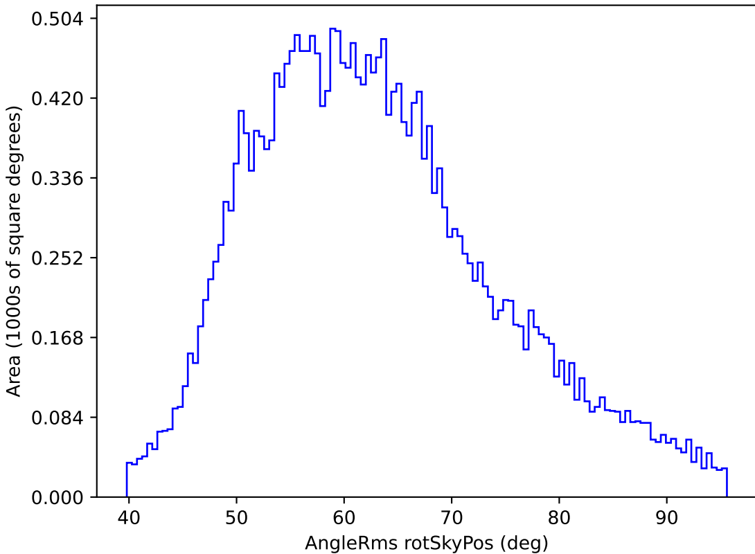
too_5_4v3.4_10yrs All sky z band: AngleRms rotSkyPos
