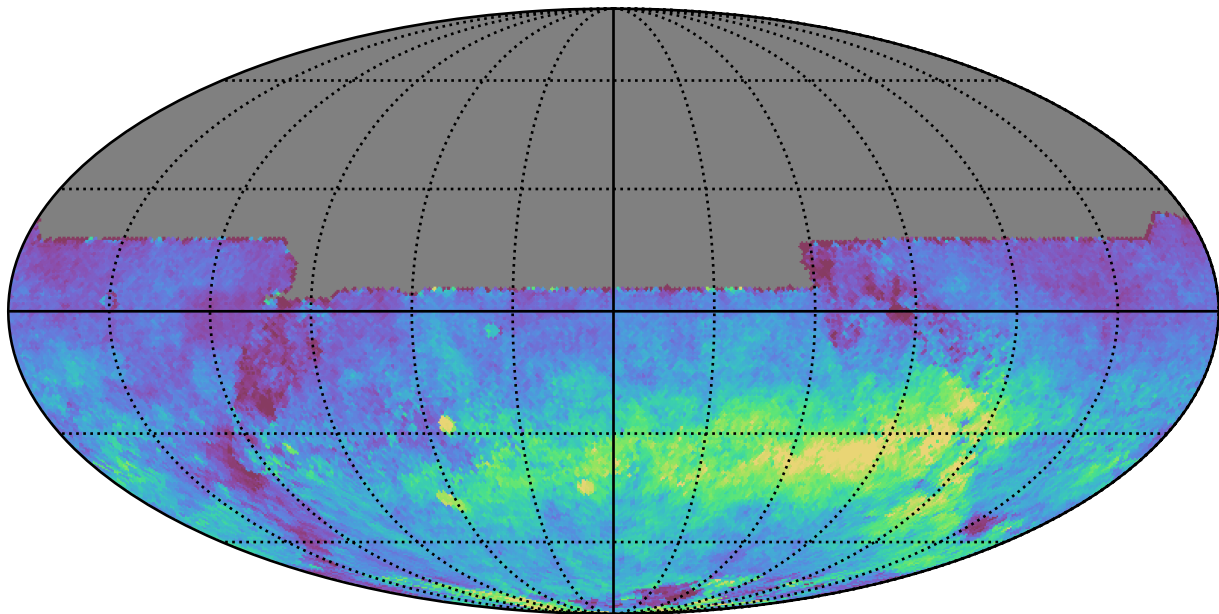
too_5_4v3.4_10yrs All sky y band: AngleRms rotSkyPos
