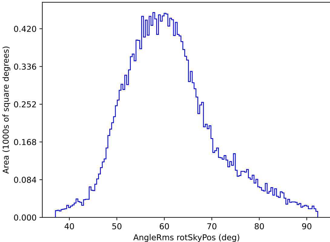
too_5_4v3.4_10yrs All sky y band: AngleRms rotSkyPos
