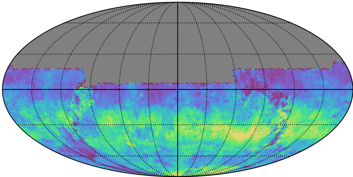
too_5_4v3.4_10yrs All sky u band: AngleRms rotSkyPos
