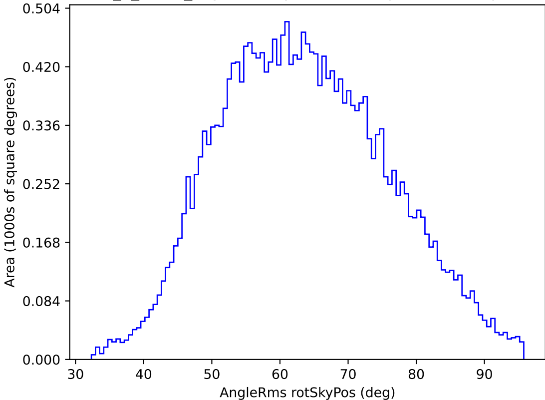
too_5_4v3.4_10yrs All sky u band: AngleRms rotSkyPos
