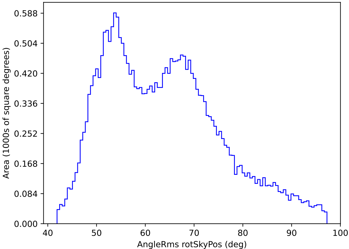
too_5_4v3.4_10yrs All sky r band: AngleRms rotSkyPos
