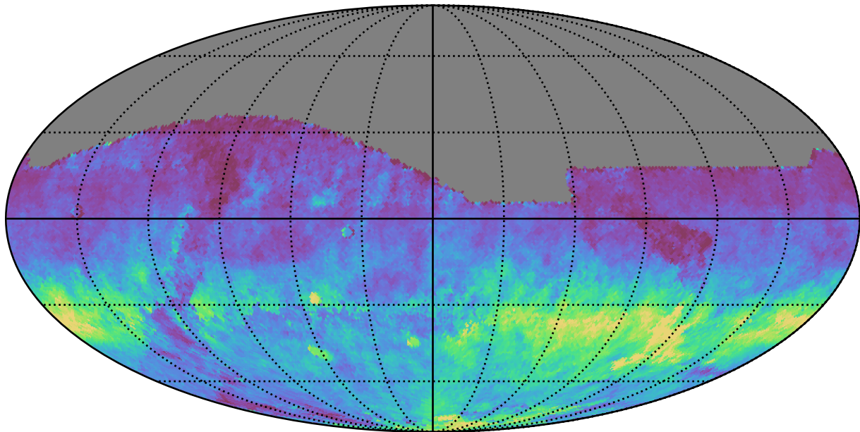
too_5_4v3.4_10yrs All sky i band: AngleRms rotSkyPos
