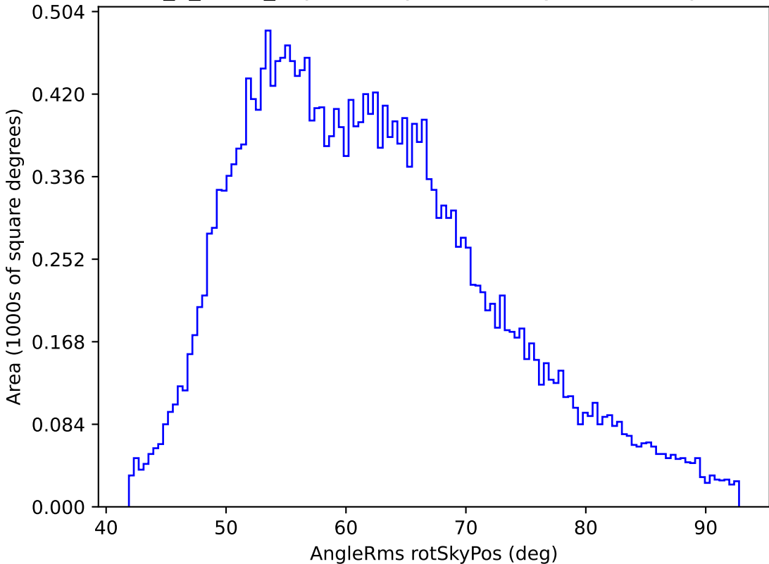
too_5_4v3.4_10yrs All sky i band: AngleRms rotSkyPos
