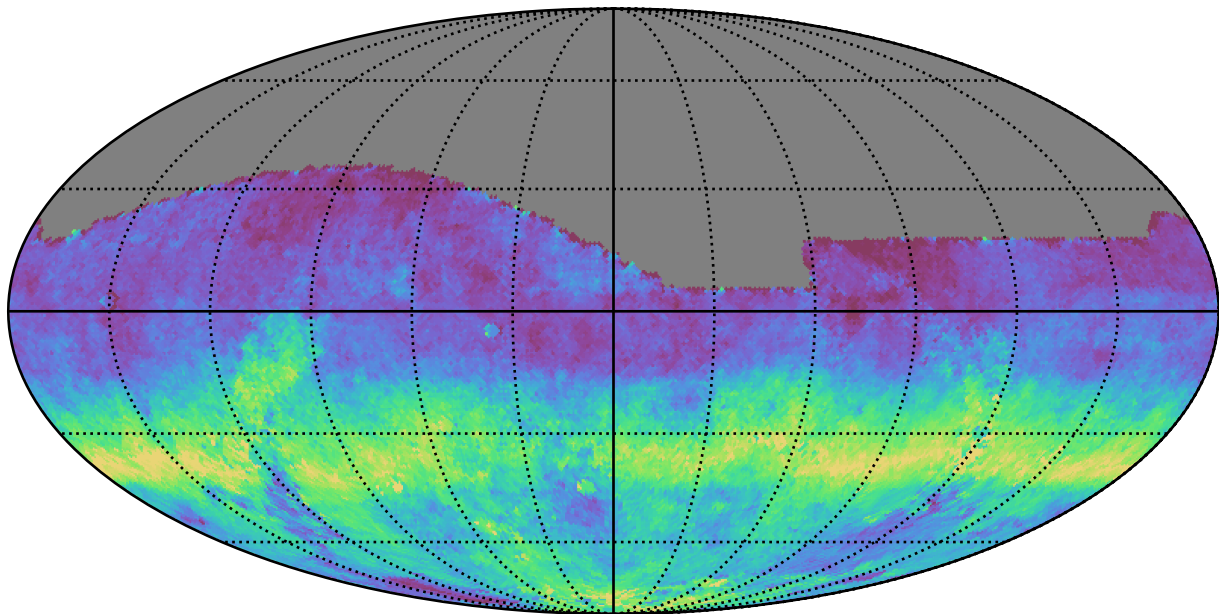
too_5_4v3.4_10yrs All sky g band: AngleRms rotSkyPos
