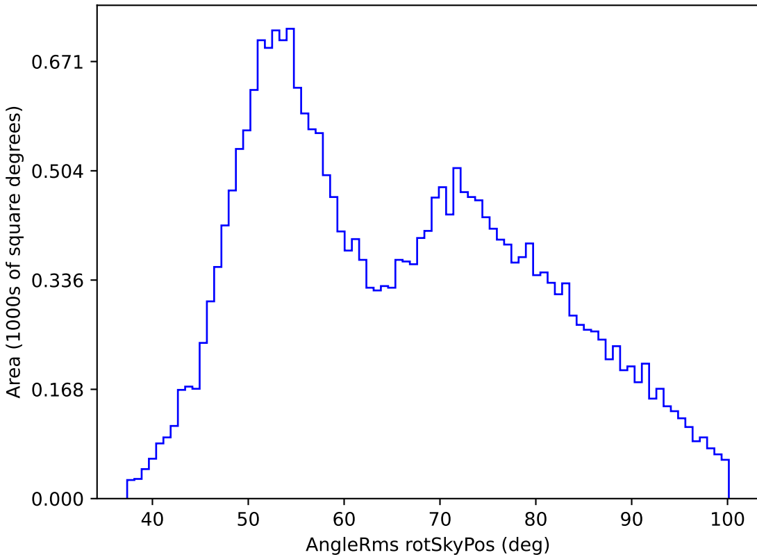
too_5_4v3.4_10yrs All sky g band: AngleRms rotSkyPos
