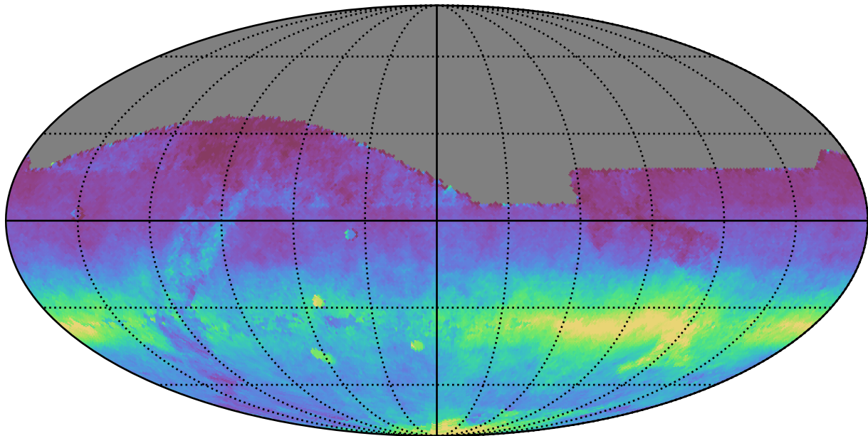
too_5_4v3.4_10yrs All sky all bands: AngleRms rotSkyPos
