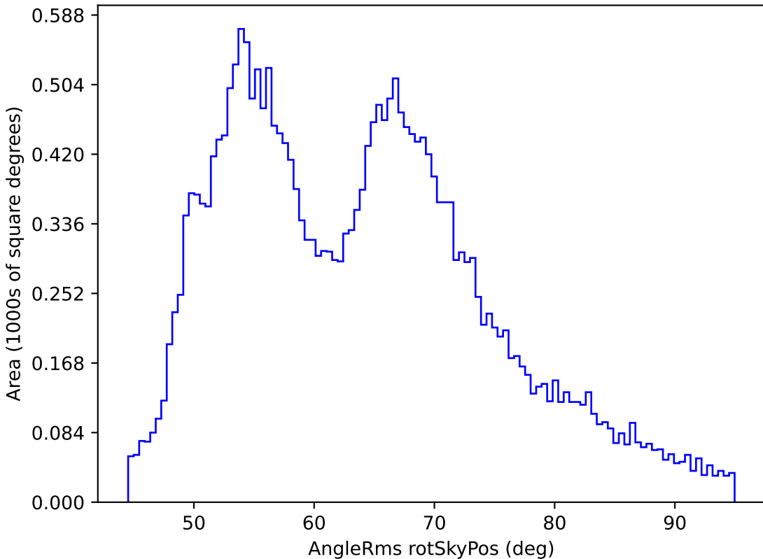
too_5_4v3.4_10yrs All sky all bands: AngleRms rotSkyPos
