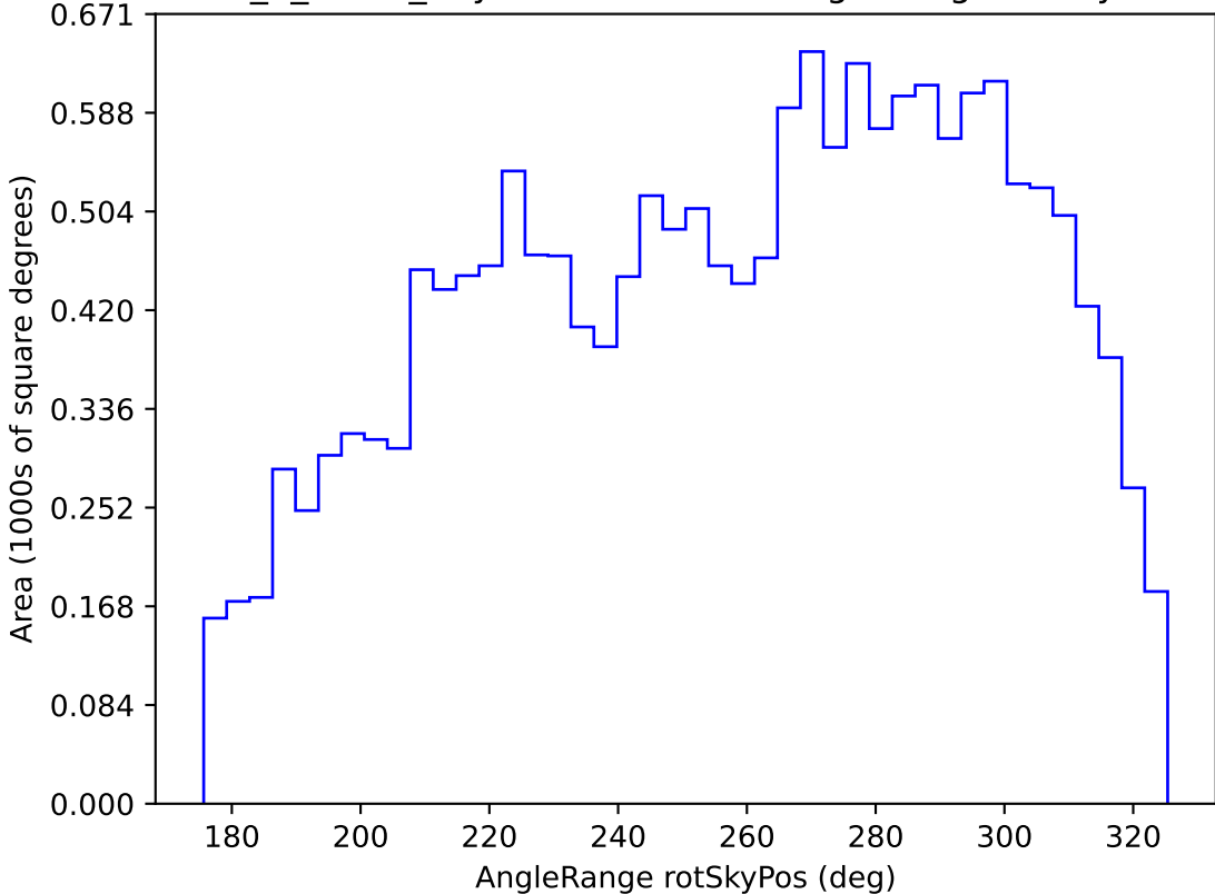
too_5_4v3.4_10yrs WFD u band: AngleRange rotSkyPos
