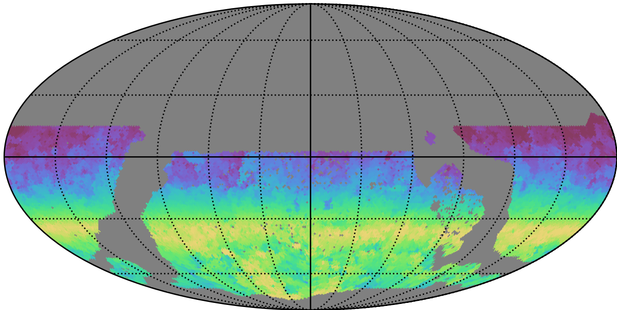
too_5_4v3.4_10yrs WFD r band: AngleRange rotSkyPos
