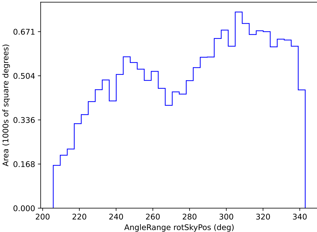
too_5_4v3.4_10yrs WFD r band: AngleRange rotSkyPos
