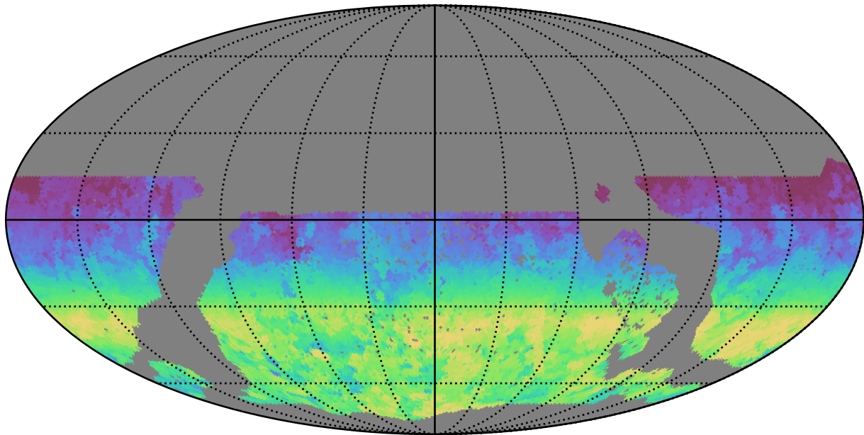
too_5_4v3.4_10yrs WFD i band: AngleRange rotSkyPos
