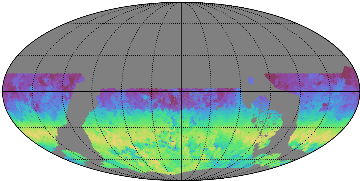
too_5_4v3.4_10yrs WFD g band: AngleRange rotSkyPos
