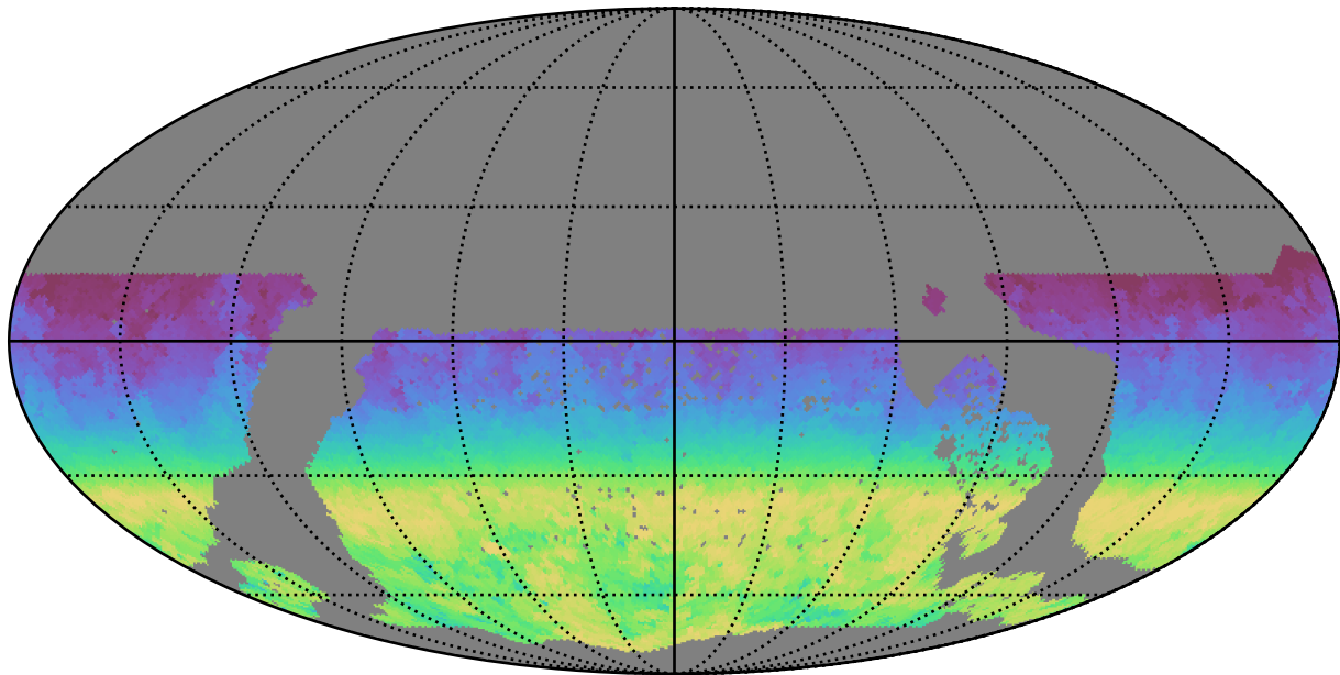
too_5_4v3.4_10yrs WFD all bands: AngleRange rotSkyPos
