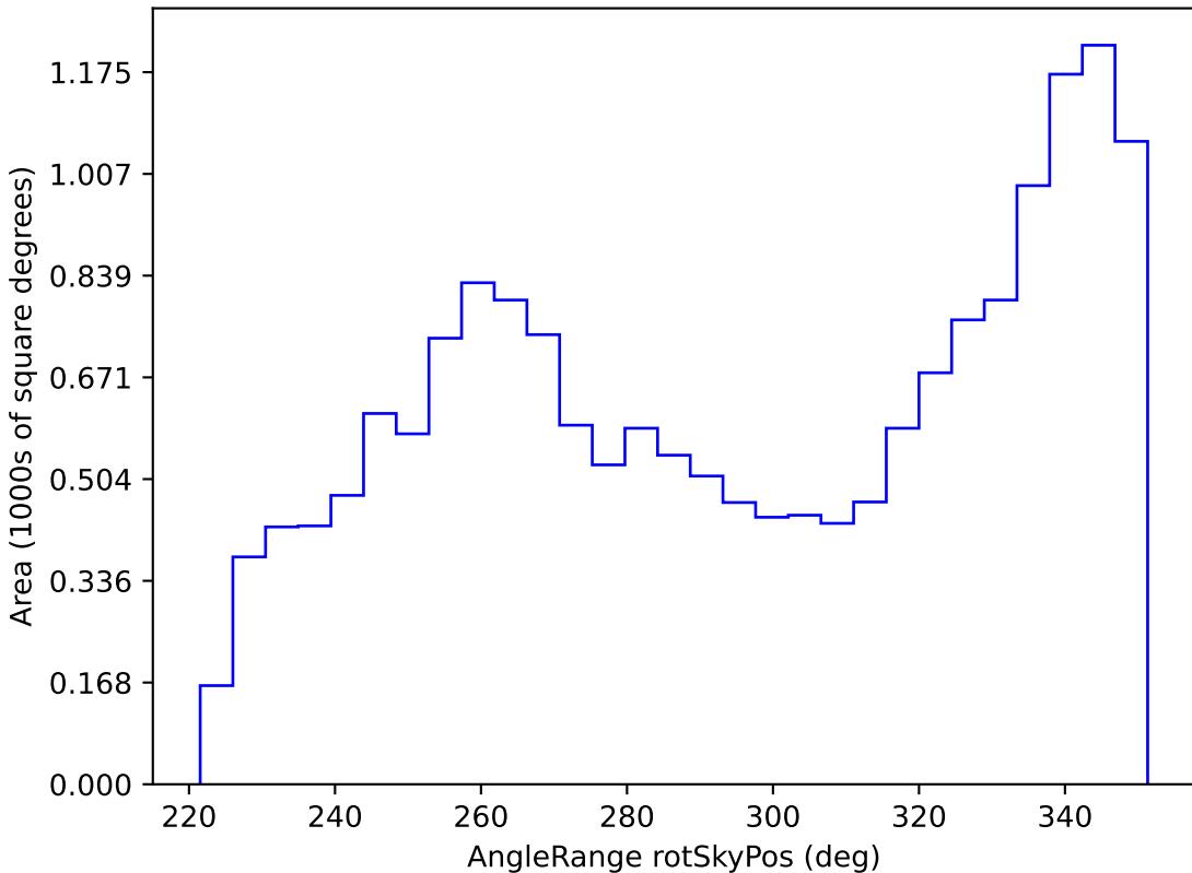
too_5_4v3.4_10yrs WFD all bands: AngleRange rotSkyPos
